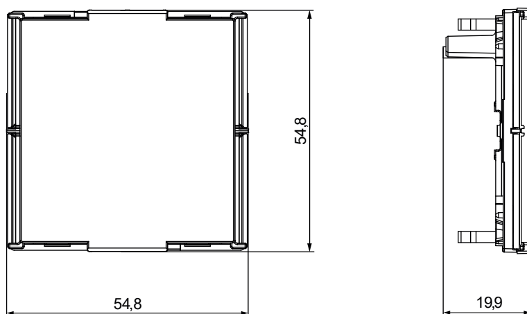
Fig. 8: KK/U4.70.1 Keypad, 1-4gang Busch-art linear®
