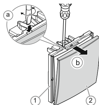
Fig. 21: Dismantling Cover
