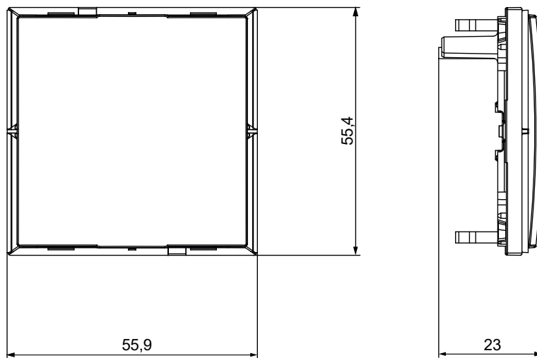
Fig. 6: KK/U4.55.1 Keypad, 1-4gang (55 mm)
