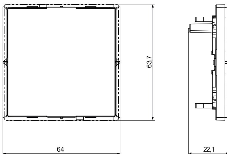
Fig. 7: KK/U4.63.1 Keypad, 1-4gang (63 mm)
