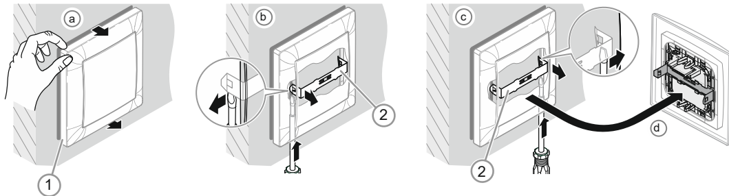
Fig. 20: Dismantling operating field of removal protection:
